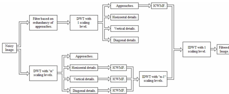
Fig. 1. Block diagram of the WDICWM algorithm.
